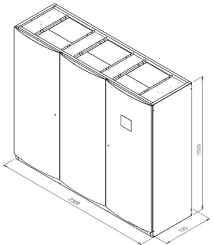
Model 130...190
